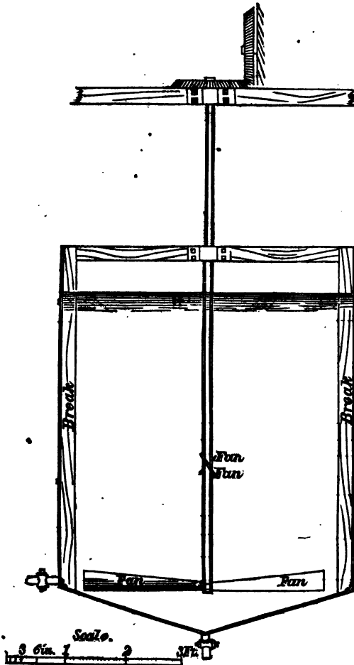
Vertical Washer.—Section.
